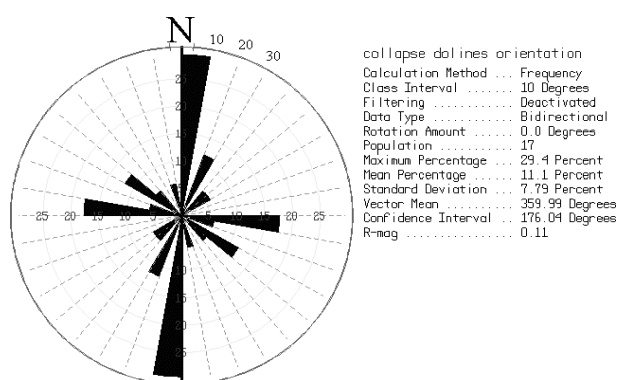
Figure 2. Rose diagram of the most common direction of collapse dolines longer axes. Longer axes are calculated regarding their direction, the longer length of axis is not calculated with stronger values.
