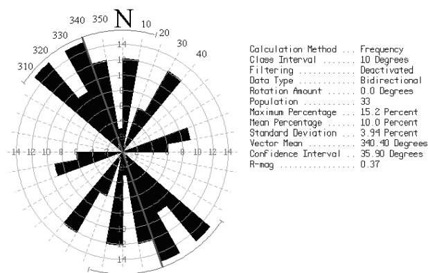
Figure 3. Rose diagram of directions of tectonic zones measured inside collapsed dolines. Data for tectonic zones were taken from ČAR, 1983; ČAR & ŠEBELA, 1997; ŠEBELA, 1994; ŠEBELA & ČAR, 2000.
